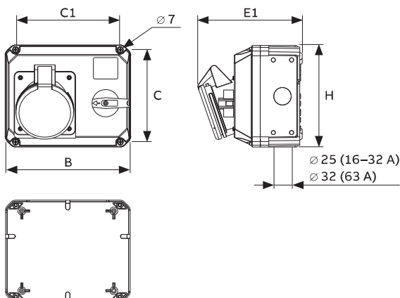
Dimensions (mm)
