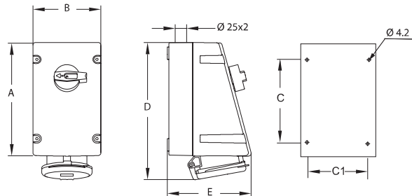
Dimensions (mm)
