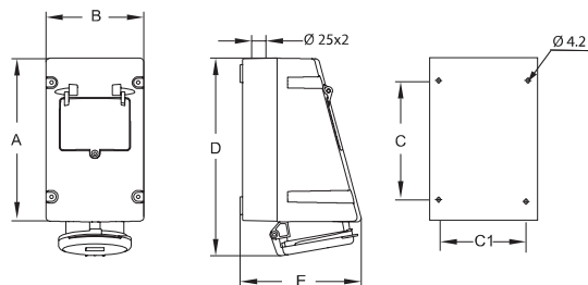
Dimensions (mm)
